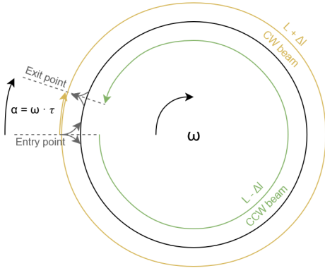
Fig. 1: Two counterpropagating light beam halves enter the fiber loop at the Entry point . Their phase is initially in sync. After transit time \tau they exit and interfere. During that time the Entry/Exit point moves according to the rotation rate \omega (by the angle \alpha = \omega \cdot \tau ). As a result the CW and CCW halves cover non-equal path lengths ( L \pm \Delta l ), which leads to a non-zero phase difference.
