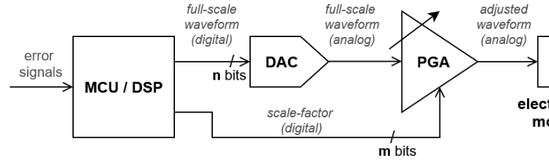
Fig. 5: Modulator with a dedicated hardware gain stage. MCU/DSP outputs a fixed-scale digital waveform, which directly drives a DAC. Then, before reaching the electro-optic actuator, scale factor of the analog waveform is adjusted with a programmable gain amplifier (PGA), or a custom gain stage, resulting in adjusted-scale waveform.
