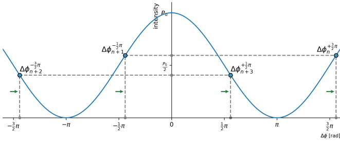
(c) Phase shift induced by positive rotation - bias points shifted right. Points \{4n, 4n+1\} correspond to higher intensity than points \{4n+2, 4n+3\} .
