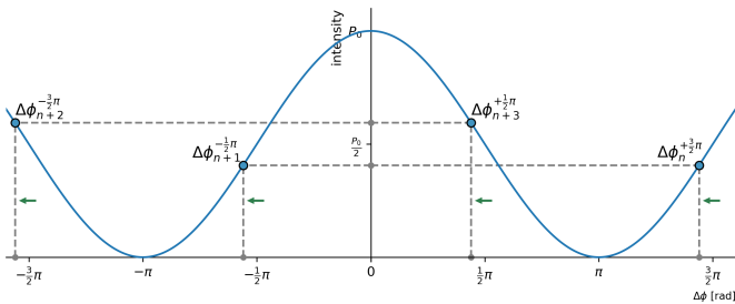
(d) Phase shift induced by negative rotation - bias points shifted left. Points \{4n, 4n+1\} correspond to lower intensity than points \{4n+2, 4n+3\} .
