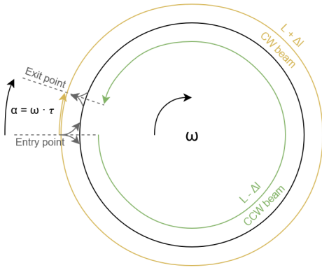
Fig. 1: Two counterpropagating light beams enter the fiber loop at the Entry point . Their phase is initially in sync. After transit time \tau they exit and interfere. During that time the Entry/Exit point moves according to the rotation rate \omega (by the angle \alpha = \omega \cdot \tau ). As a result the CW and CCW beams cover non-equal path lengths ( L \pm \Delta l ), which leads to a non-zero phase difference.
