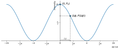
Fig. 2: Optical circuit response is a shifted cosine. The two exemplary operating points refer to the circuit being at rest, yielding the maximum possible intensity - (0, P_0) - and subjected to rotation, at non-zero phase shift and decreased intensity - (\Delta\phi, P(\Delta\phi)) .
