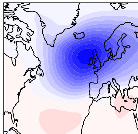
IPSL-CM6A-LR
