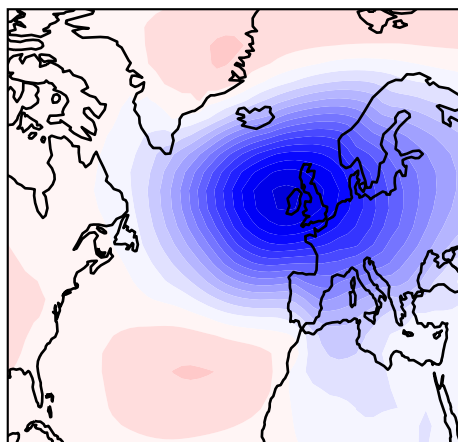
HadGEM3-GC31-LL
