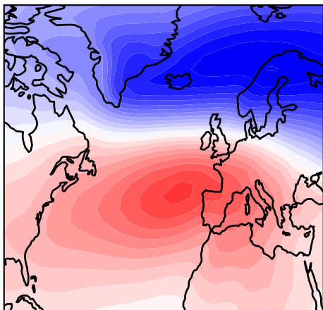
HadGEM3-GC31-LL
