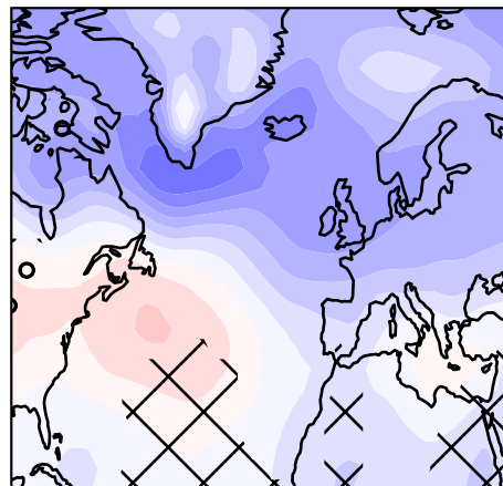
IPSL-CM6A-LR
