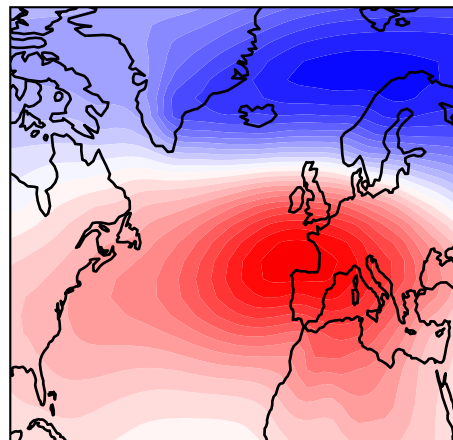
IPSL-CM6A-LR
