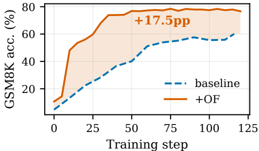
(a) Dense (Qwen2.5-3B)
