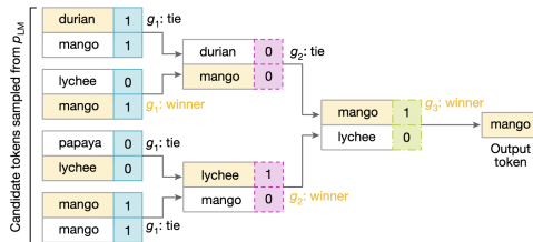
Tournament sampling: over-generation with watermark-based iterative selection
