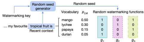
LLM probabilities and random watermarking functions
