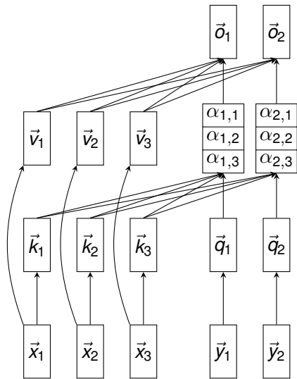
Cross-attention
