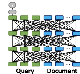
1 (c) All-to-all Interaction (e.g., BERT)
