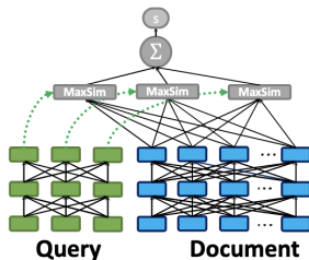
(d) Late Interaction (i.e., the proposed COLBERT)
