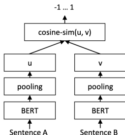
Inference (Individual Encoders)
