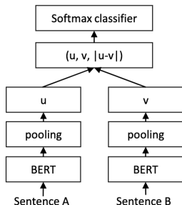
Training (Shared weights)
