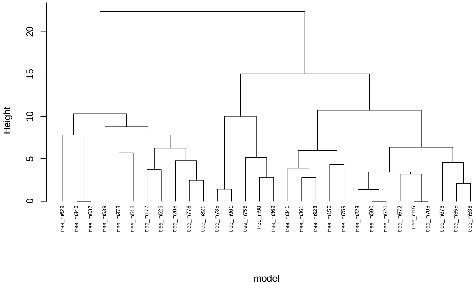
VIC dendrogram -- bs (manhattan)
