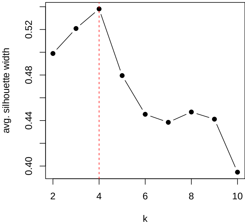
Behavioural -- bs (manhattan)
