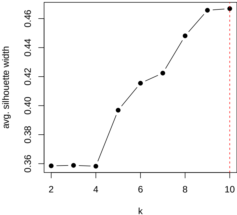
Behavioural -- cs (euclidean)
