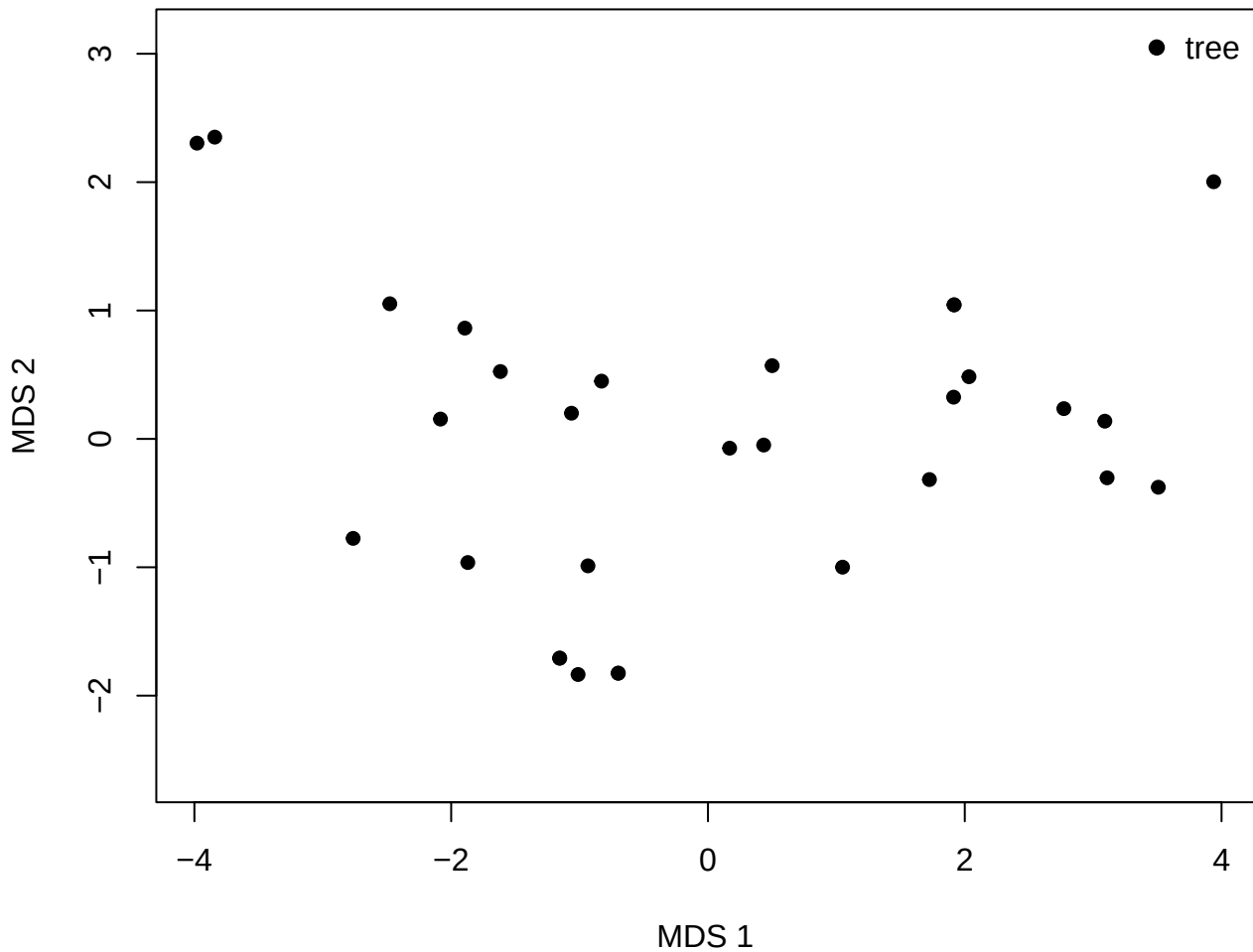
VIC MDS -- bs (euclidean)
