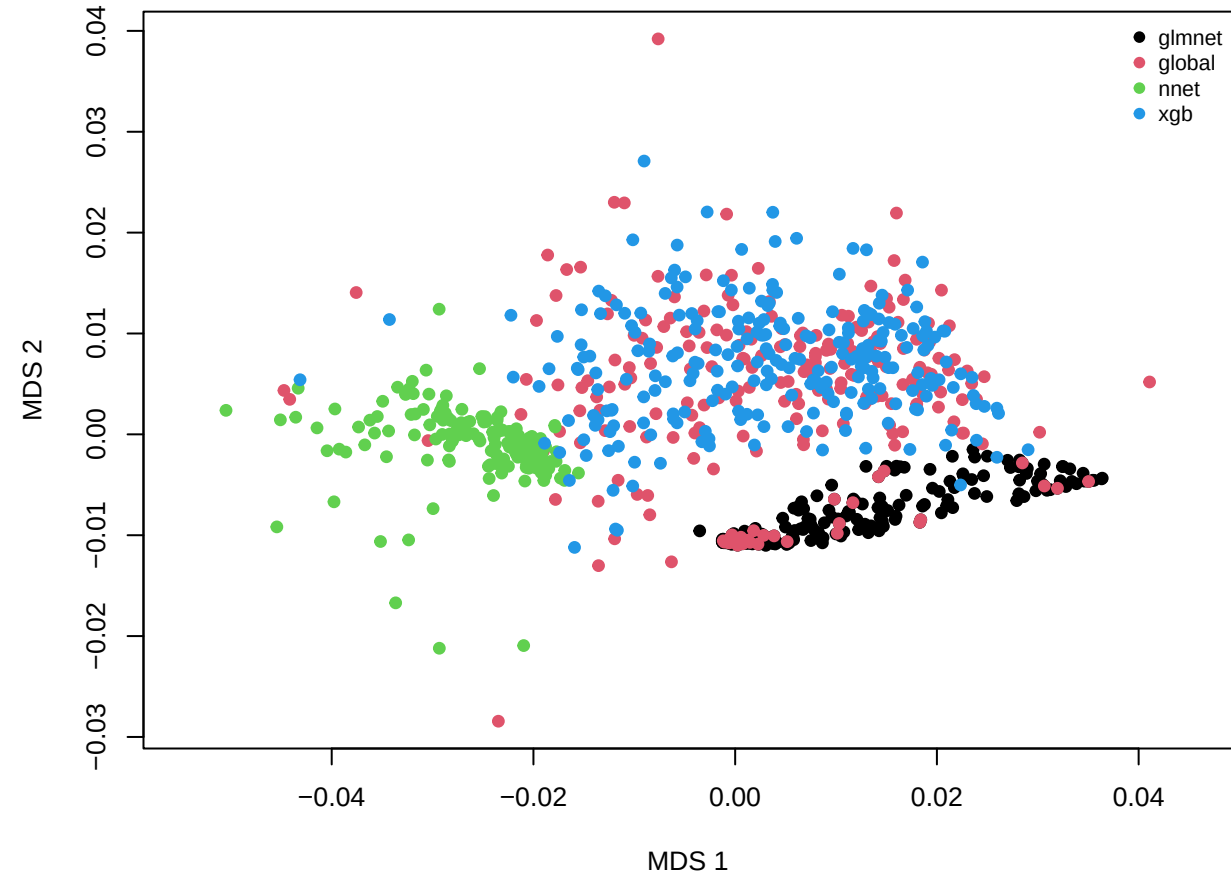
VIC -- PAM cluster ( k^* = 5 )
