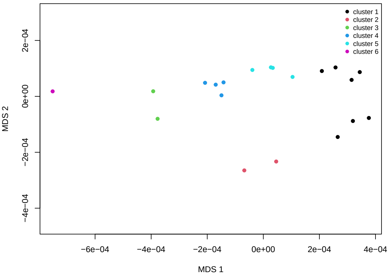
Behavioural -- PAM cluster ( k^* = 6 )
