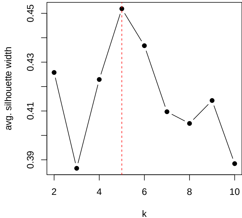
VIC -- cs (manhattan)
