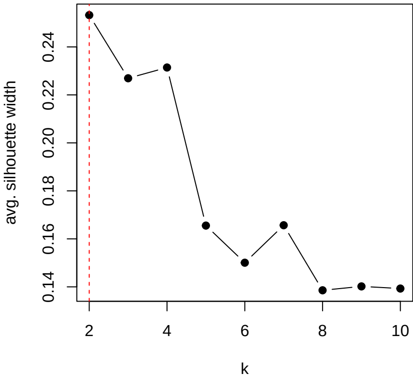
Behavioural -- st (manhattan)
