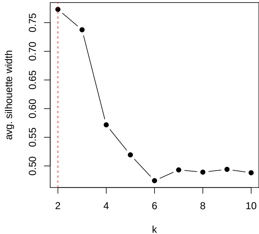
VIC -- st (manhattan)
