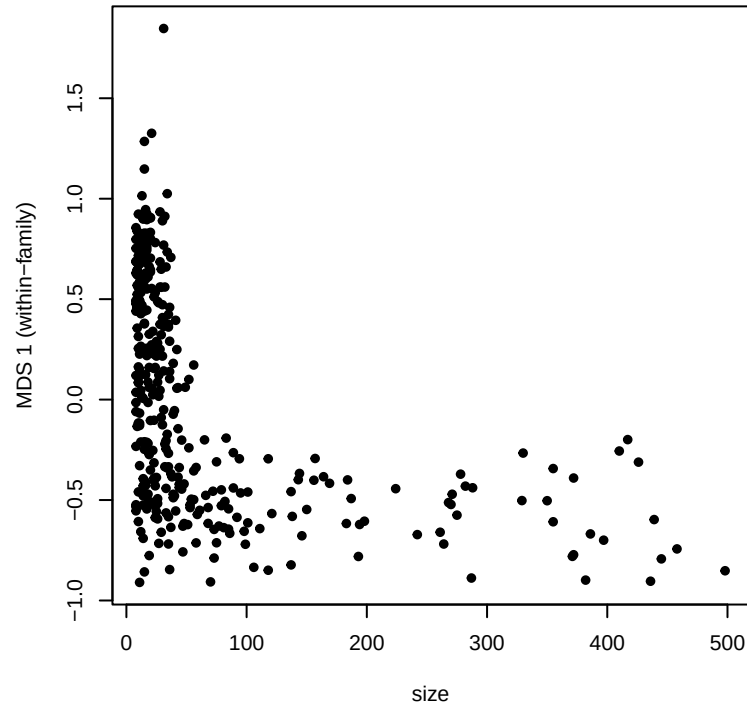
st / nnet
