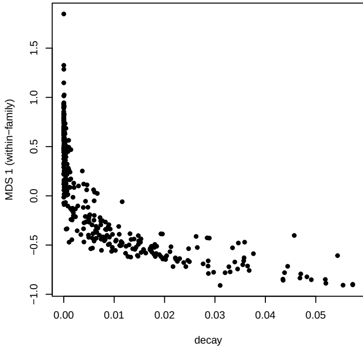
st / nnet
