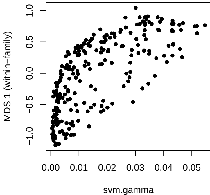
st / svm.radial
