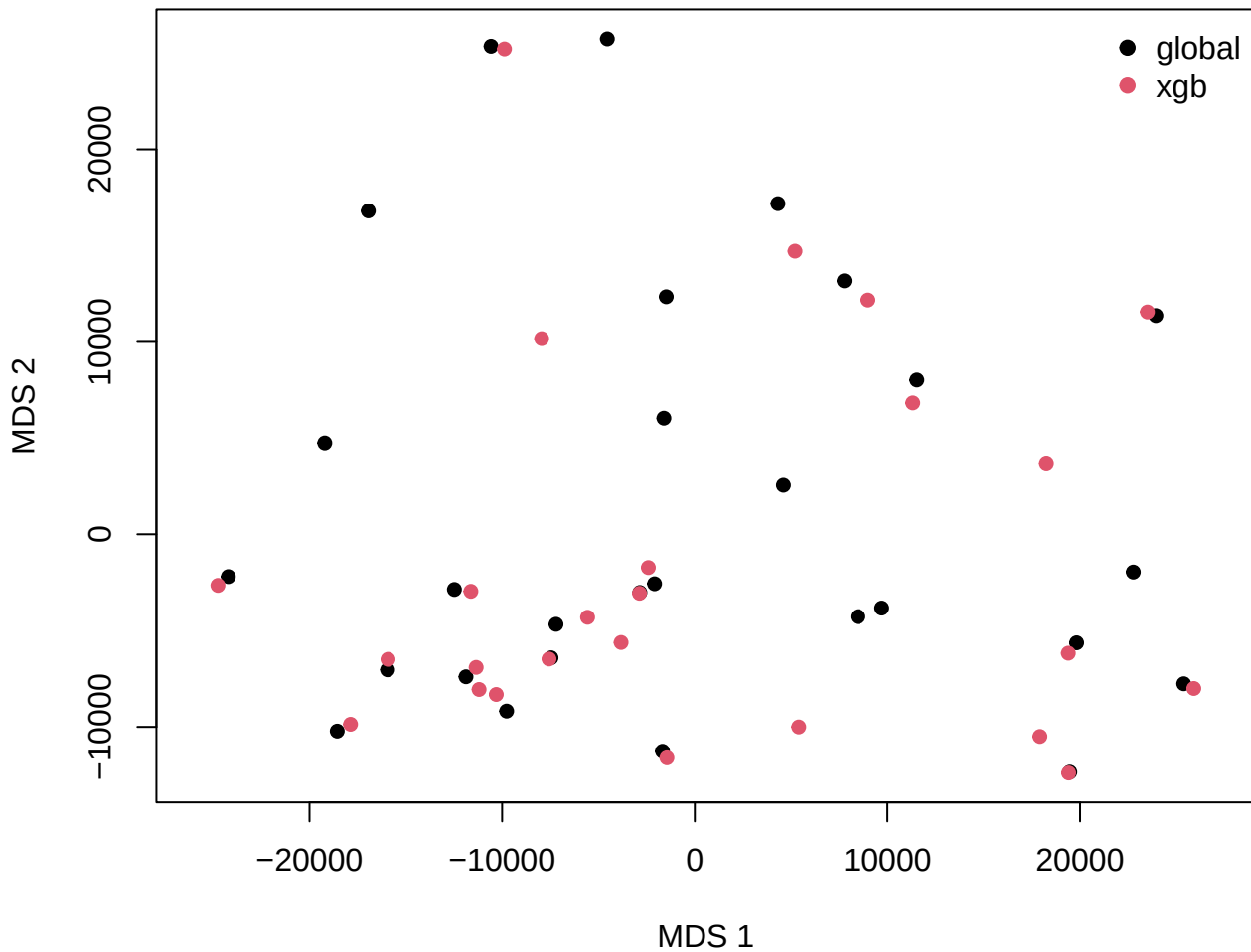
Classical MDS -- bs (manhattan)
