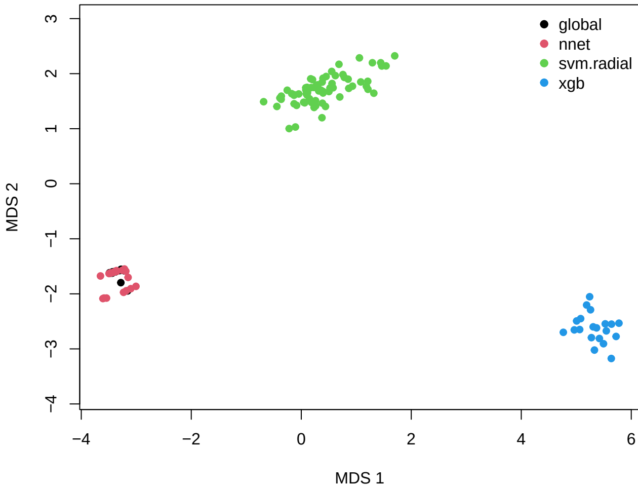
Classical MDS -- cr (manhattan)
