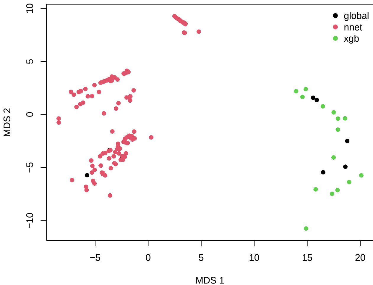
Classical MDS -- gc (manhattan)
