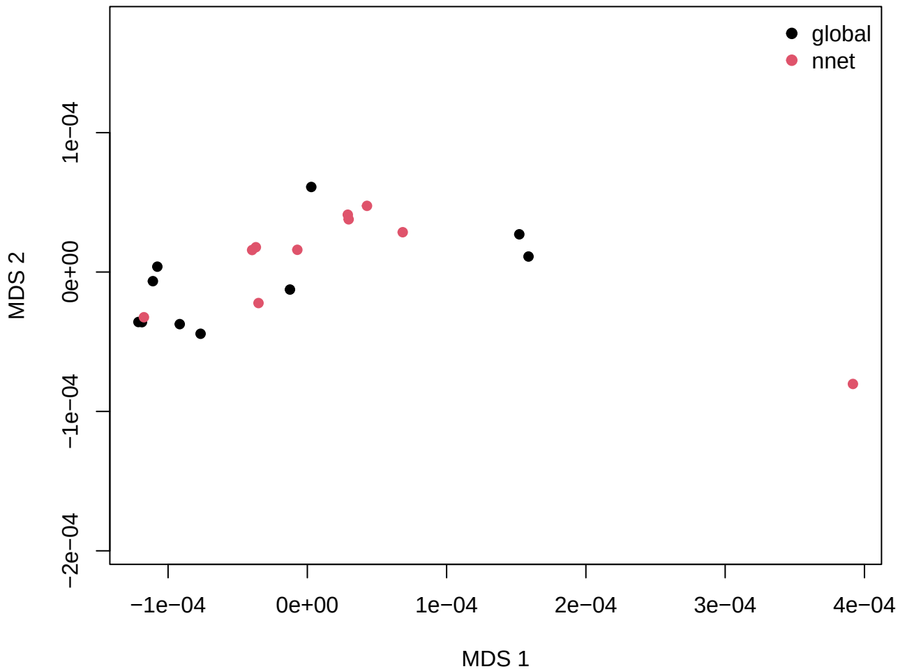
Classical MDS -- mk (euclidean)
