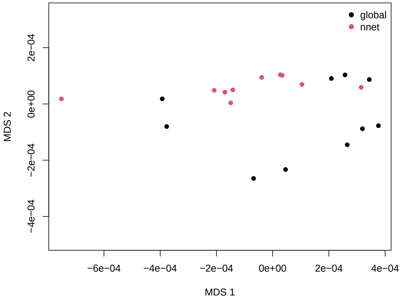
Classical MDS -- mk (manhattan)
