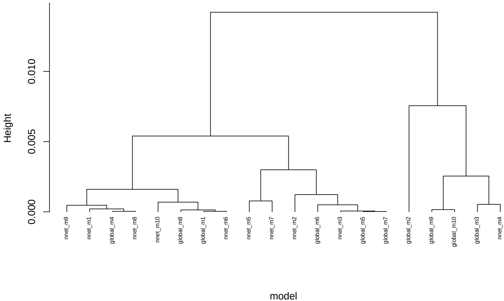
VIC dendrogram -- mk (euclidean)
