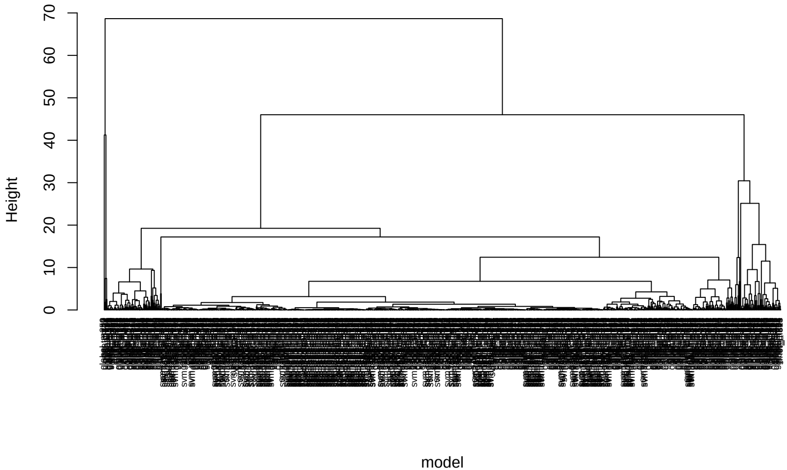
VIC dendrogram -- st (manhattan)
