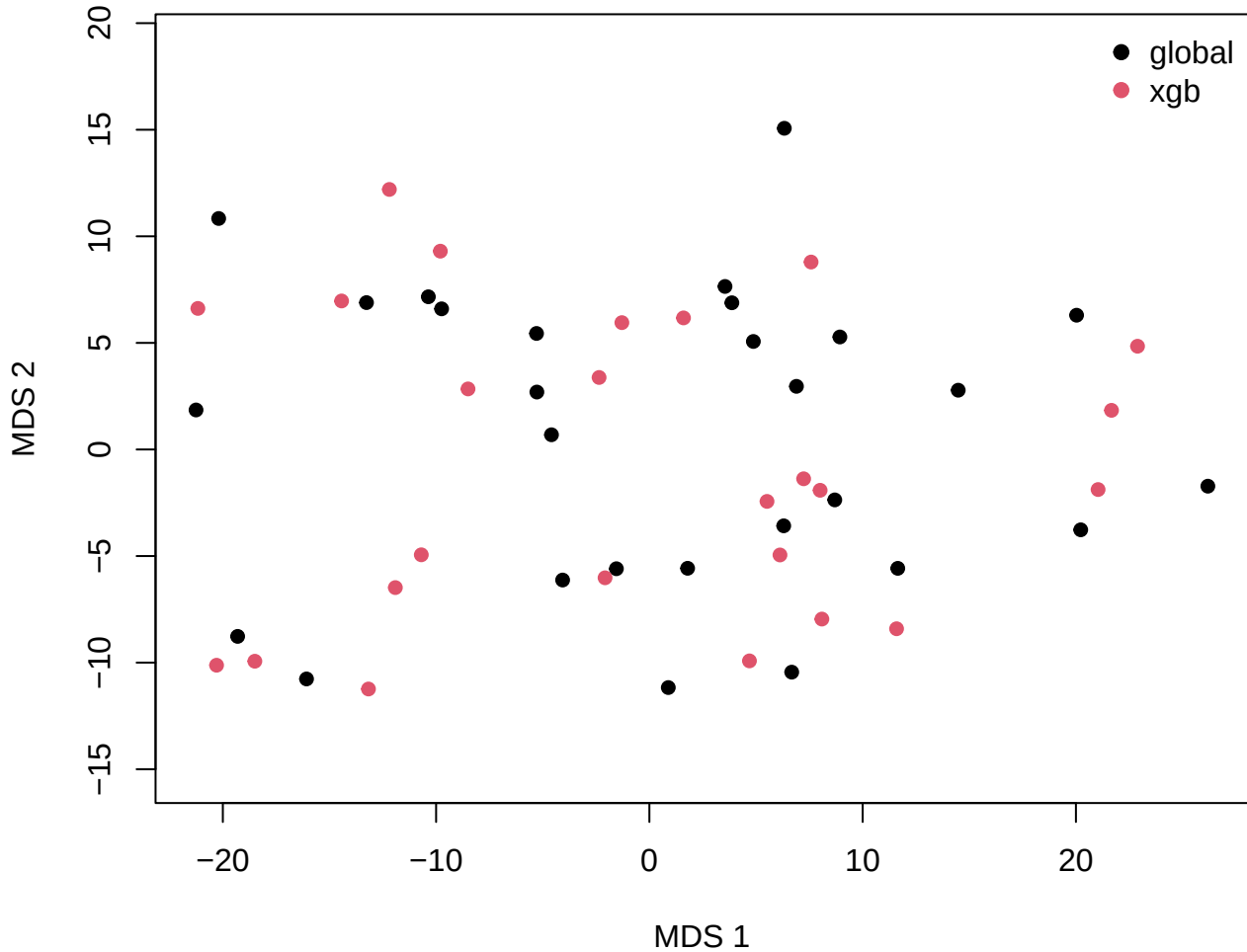
VIC MDS -- bs (manhattan)
