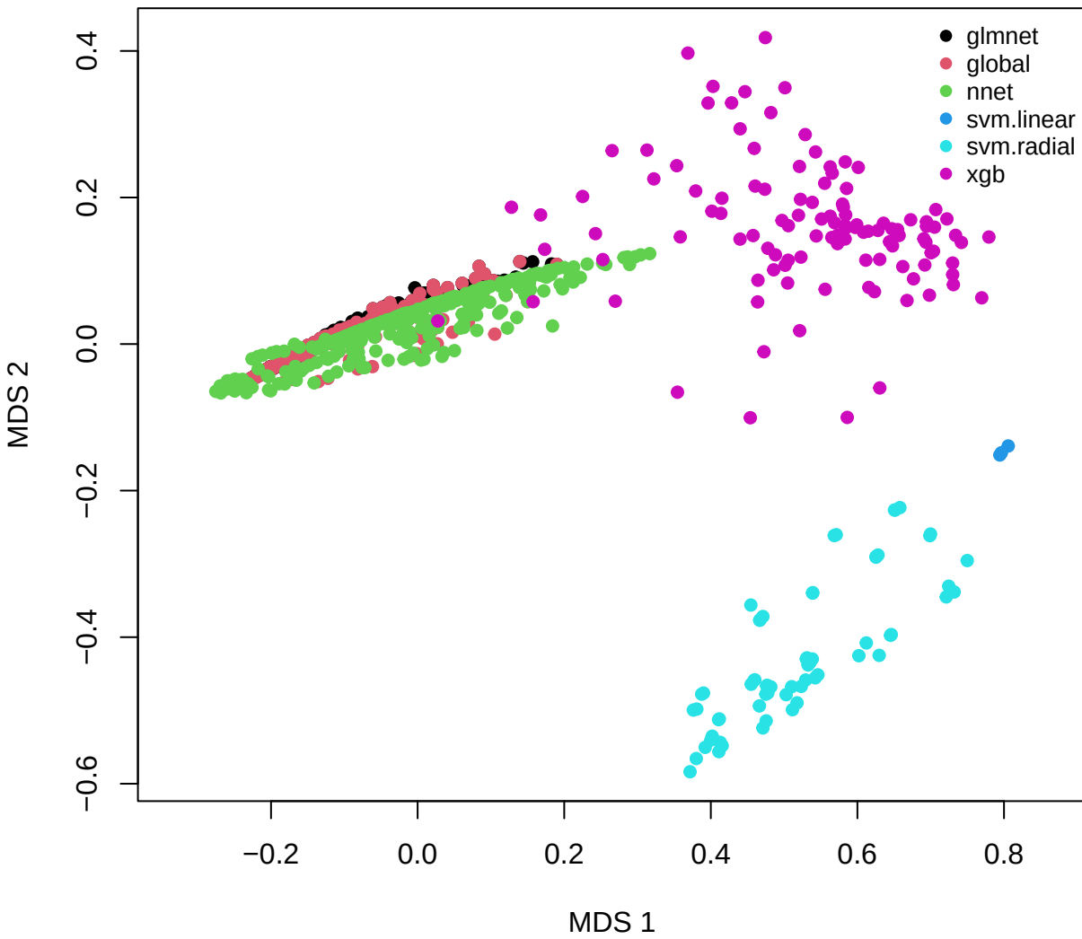
Behavioural distance -- bc
