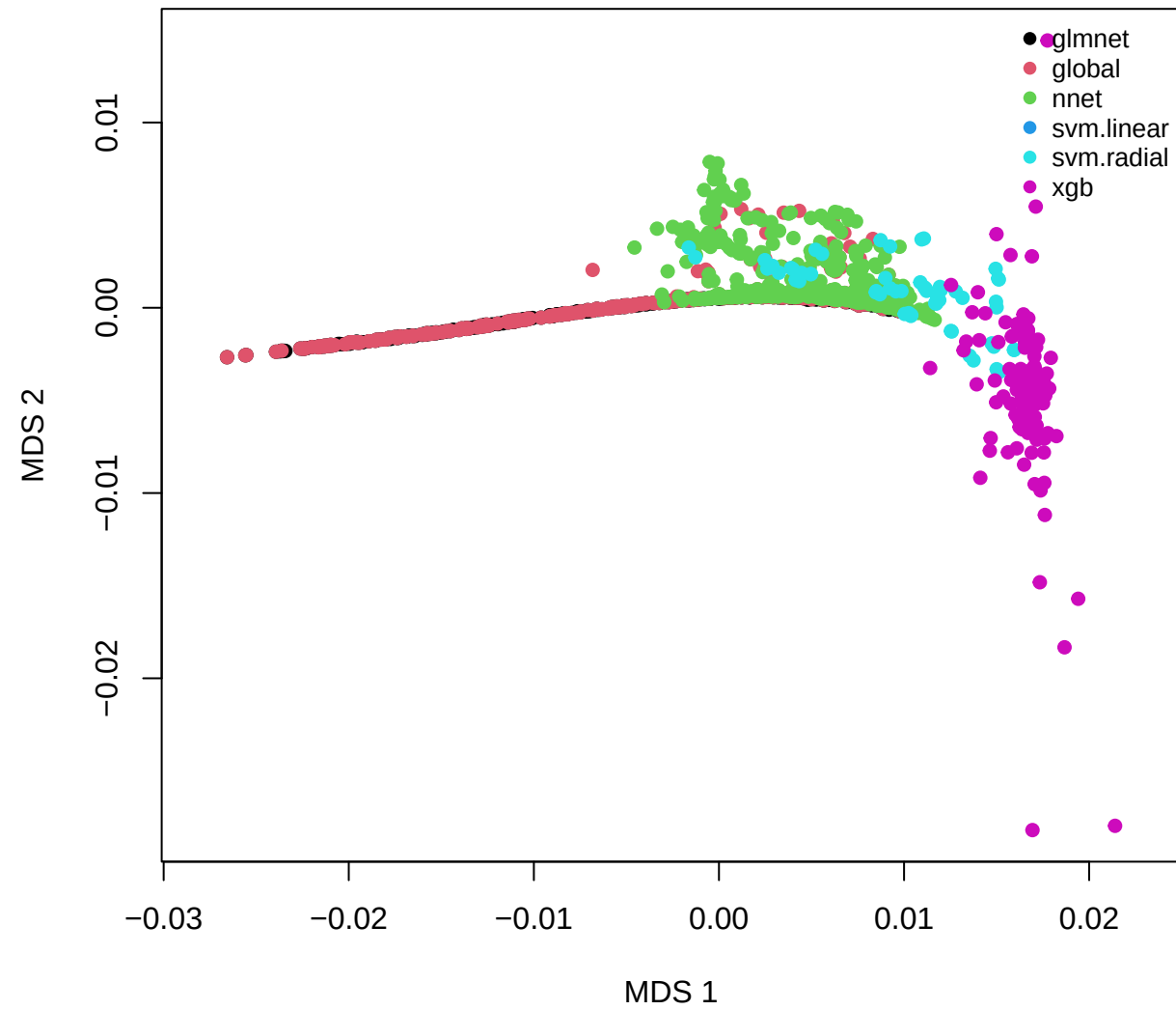
VIC distance -- bc
