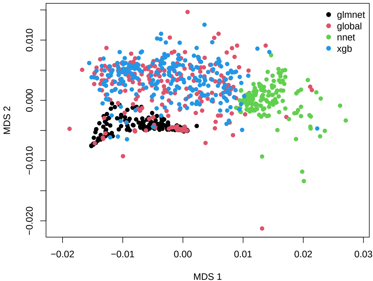
VIC MDS -- cs (euclidean)
