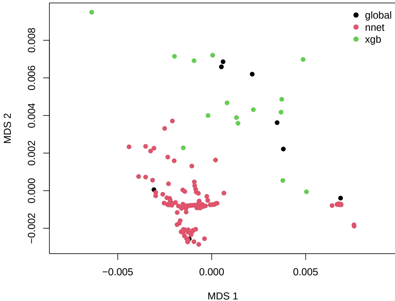
VIC MDS -- gc (euclidean)
