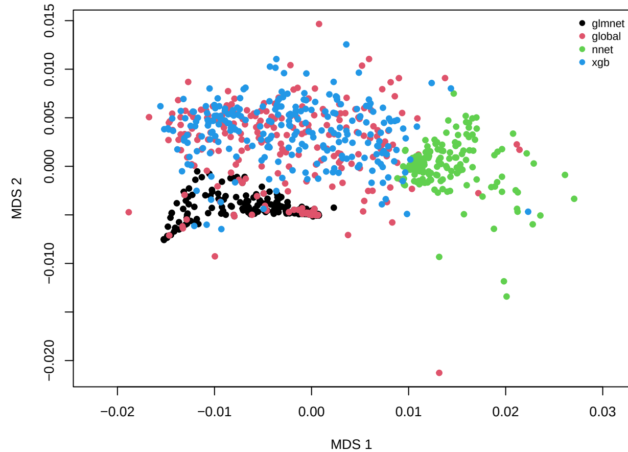
VIC -- PAM cluster ( k^* = 5 )
