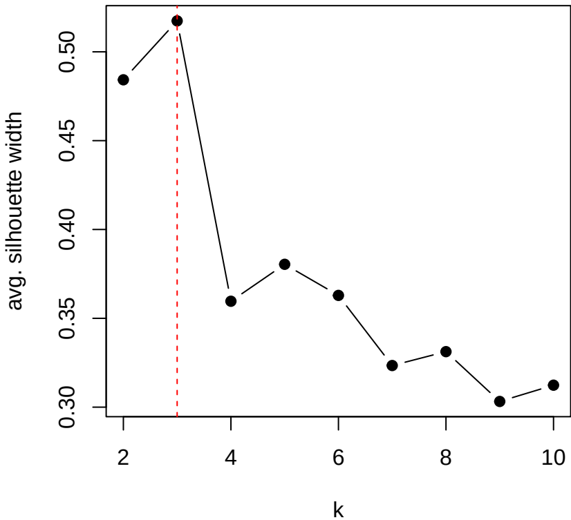
Behavioural -- cs.bin (manhattan)
