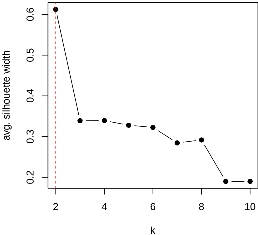
Behavioural -- fc.bin (manhattan)
