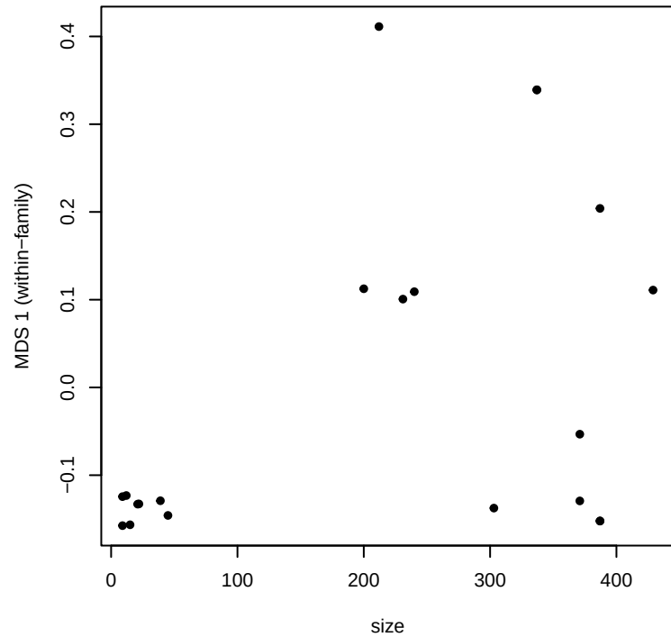
gc / nnet
