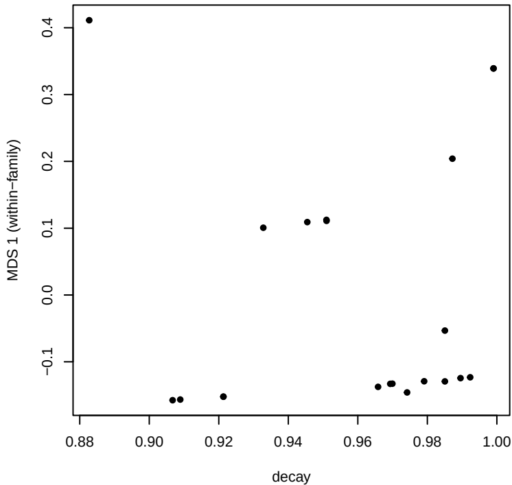
gc / nnet
