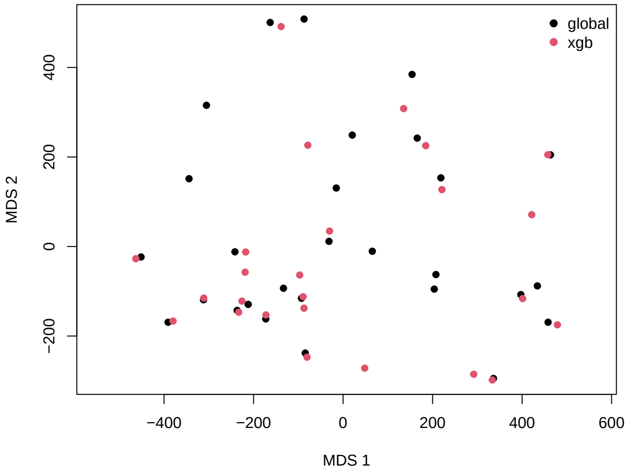
Classical MDS -- bs (euclidean)
