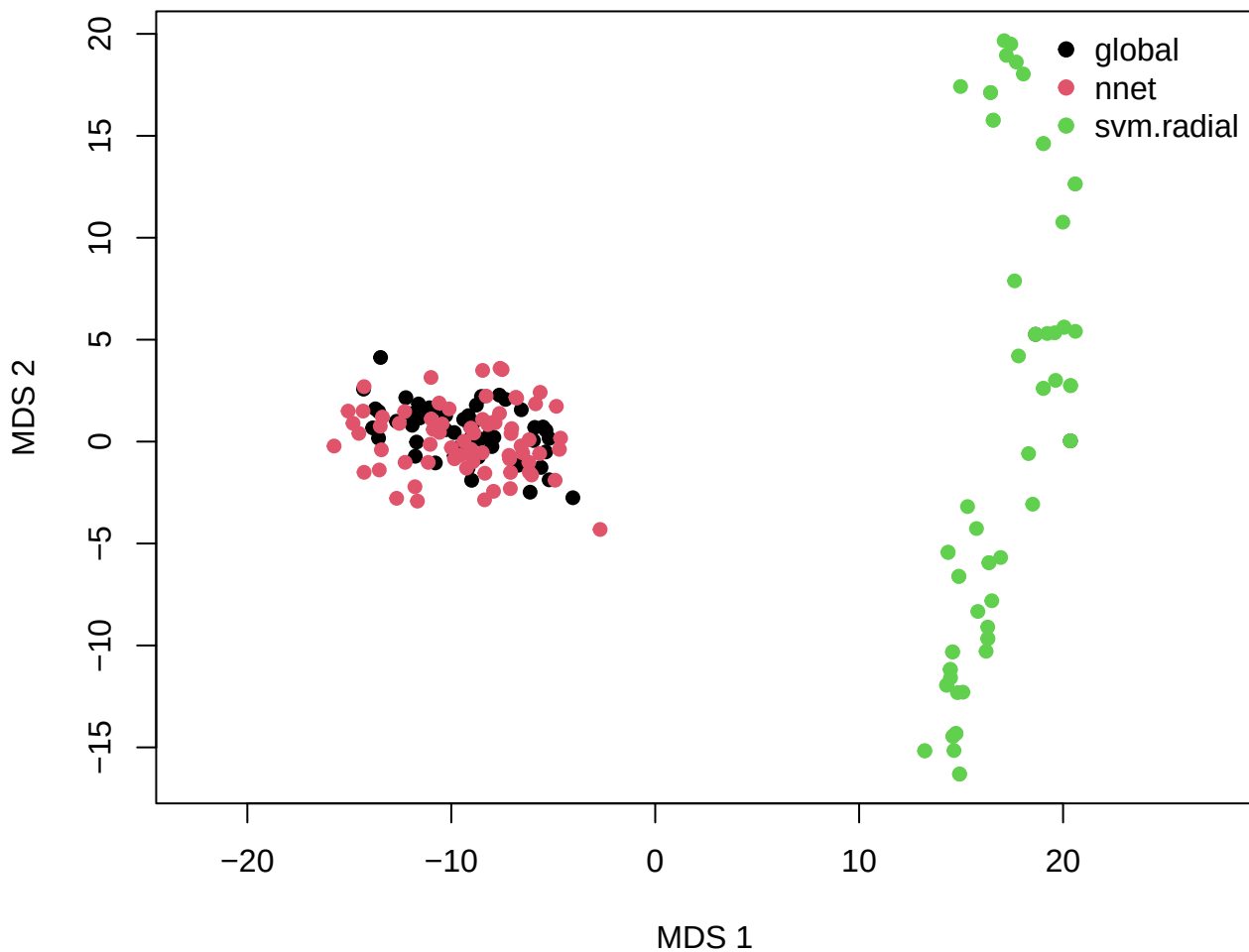
Classical MDS -- st (manhattan)
