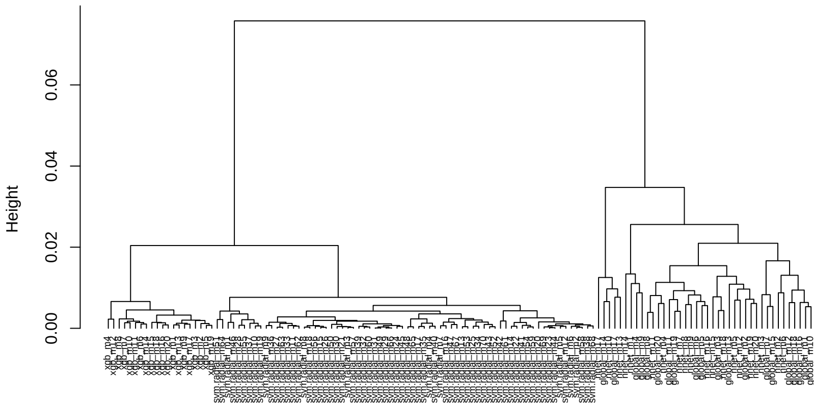
VIC dendrogram -- cr (euclidean)
