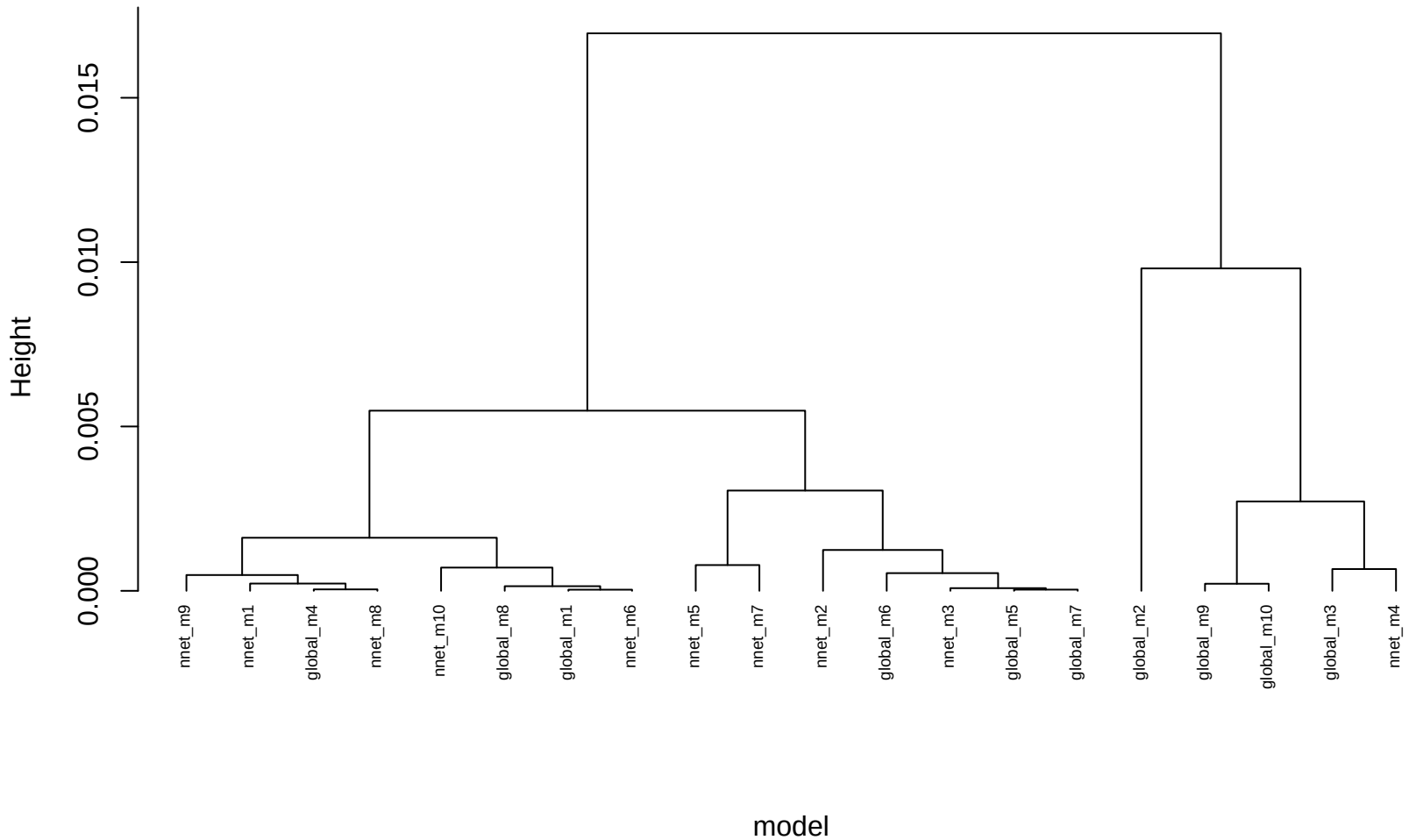
VIC dendrogram -- mk (manhattan)
