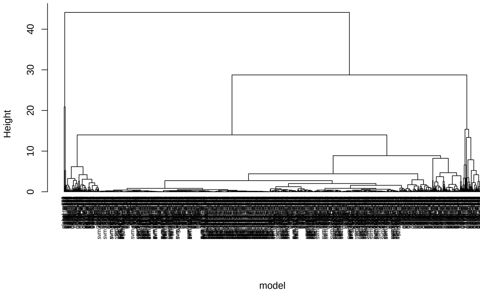
VIC dendrogram -- st (euclidean)
