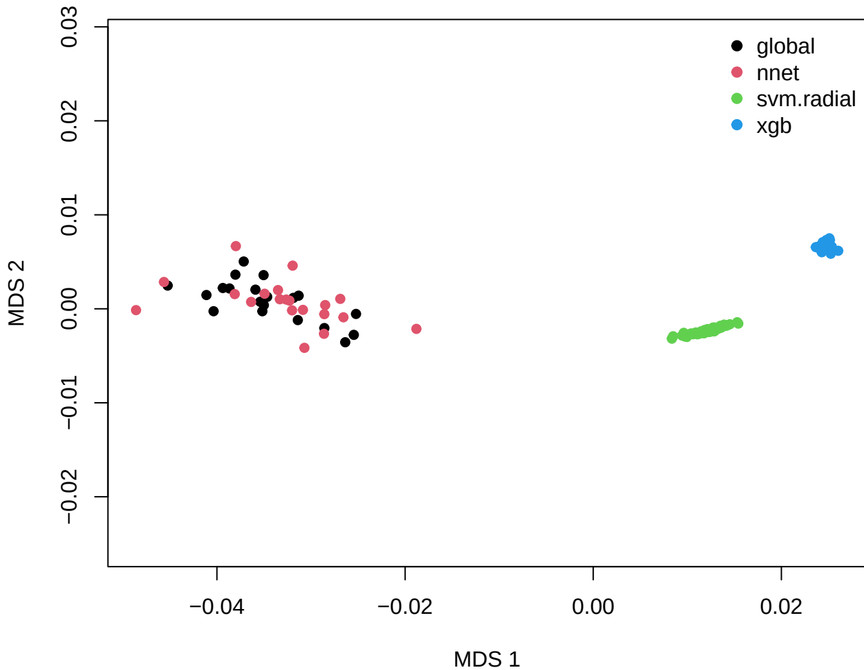
VIC MDS -- cr (euclidean)
