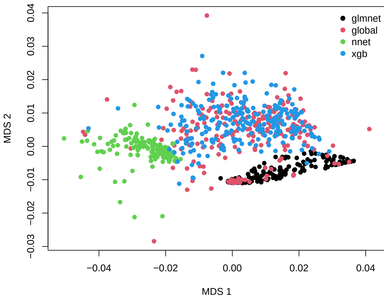
VIC MDS -- cs (manhattan)
