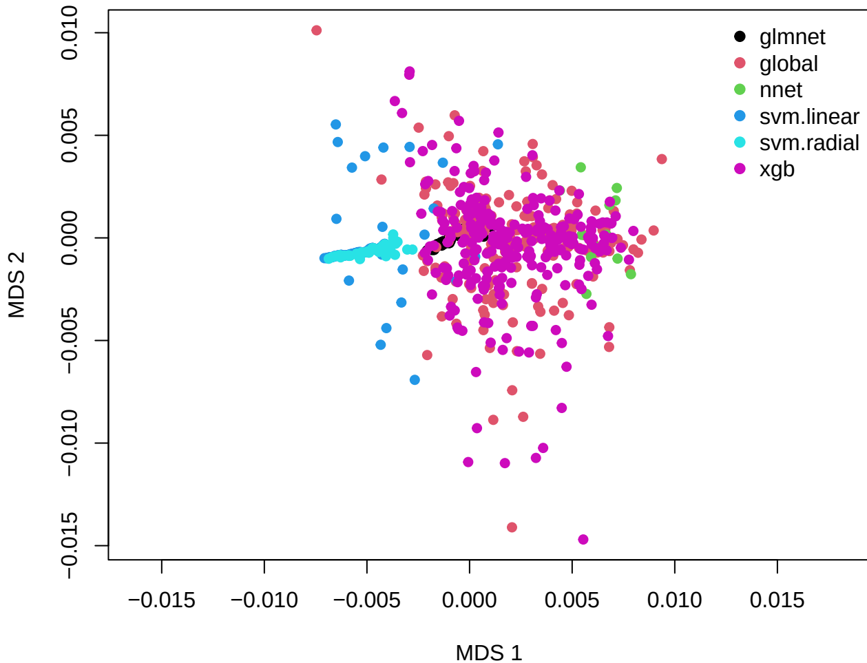
VIC MDS -- fc.bin (euclidean)
