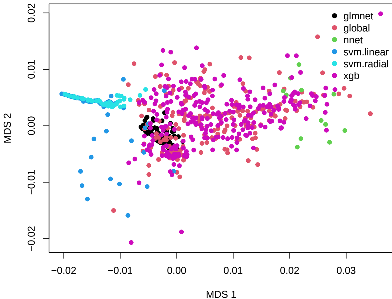
VIC MDS -- fc.bin (manhattan)
