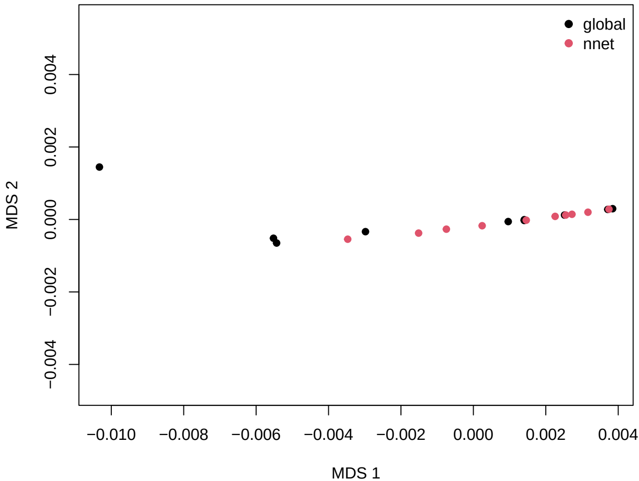
VIC MDS -- mk (euclidean)
