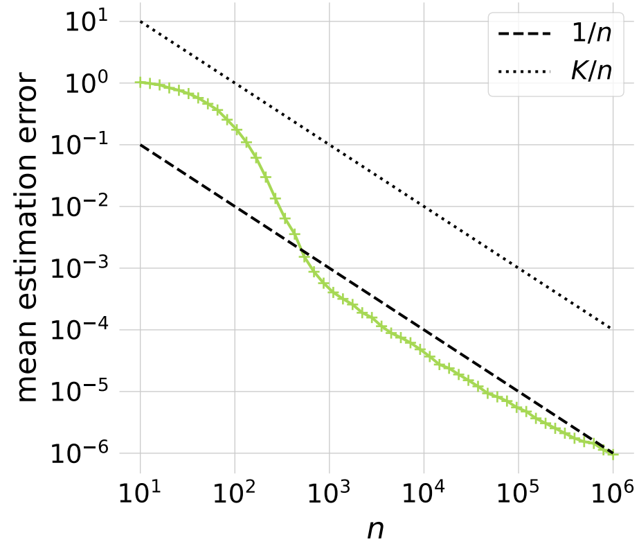
Feature x_2
