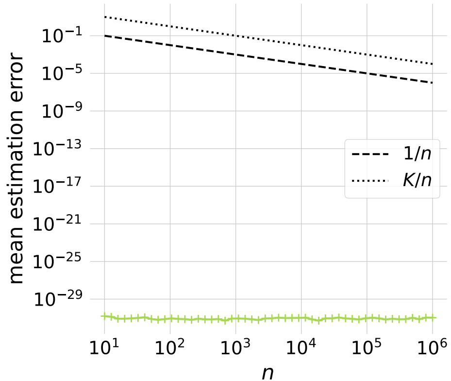
Feature x_3
