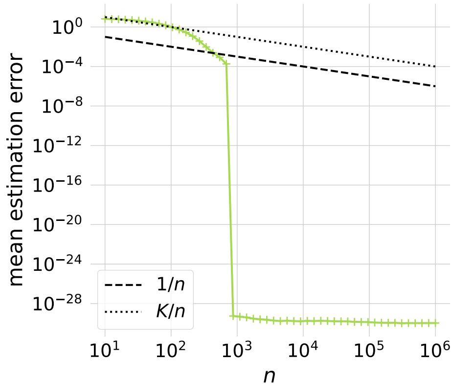
Feature x_4
