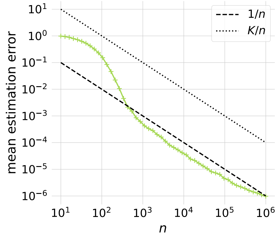
Feature x_1
