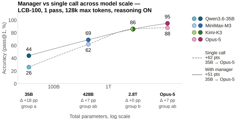
Figure 6: Accuracy by model scale, reasoning on, 128k, one pass . The same numbers as Figure 5a, against parameter count. Dashed = single call, solid = with manager; the block under each tick gives that model’s \Delta and Tukey group, and the legend each arm’s gain from the smallest to the largest.
