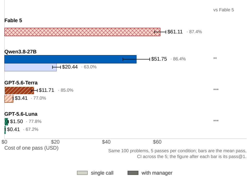
Figure 3: The scaffold’s bill. Cost of one pass over the same 100 problems; Table 1 is the arithmetic behind every bar. No cached-input discount is taken, and Qwen3.8-27B is priced at OpenRouter market rates. The top bar of each pair is the manager, dark; the single call is under it, light; all are at a 128k output cap, and hatch is the model. The right-hand column tests each top bar against Fable 5’s single call (Welch per run, n = 5 vs 5; Holm-corrected across seven comparisons): * p < .05 , ** p < .01 , *** p < .001 . Unbracketed comparisons: each manager – single increase is significant ( 8.7 \times 10^{-5} or better per run, < 3.5 \times 10^{-5} per problem); GPT-5.6-Luna’s manager undercuts GPT-5.6-Terra’s single call by $1.91 ( 2.1 \times 10^{-7} per run, < 3.5 \times 10^{-5} per problem). At 1.18x the assumed Qwen rate ($0.413/$3.25 per MTok, inside the spread across hosted providers) the manager’s cost advantage over Fable 5 disappears entirely — a larger uncertainty than any p-value here.
