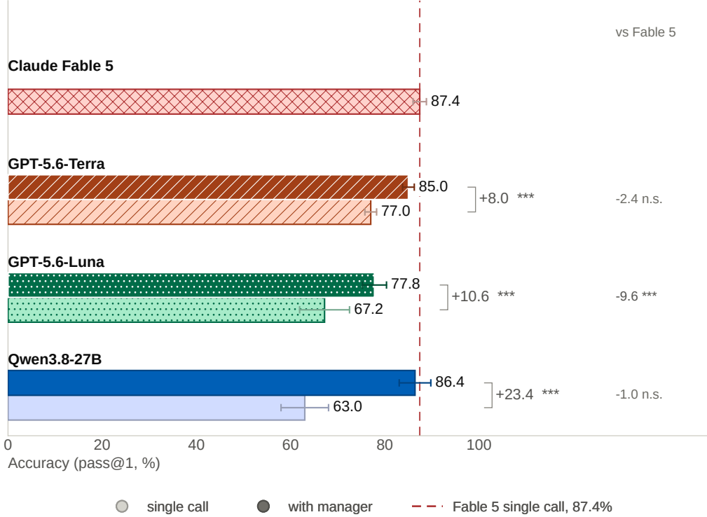
Figure 2: Manager vs. single call. 128k \times 5 passes, reasoning on. Bars are pass@1 on the same 100 problems, the line through each the 95% CI across the 5 passes ( t , df = 4 ). The top bar of each pair is the manager, dark; the single call is under it, light; hatch is the model. “Single call” is one call with no tools and no loop; Fable 5 ran single-only, so it has one bar, which the dashed rule carries across the chart. The bracket beside each pair is manager – single call; the right-hand column tests the top bar against Fable 5. Both are paired sign-flip permutation tests, unit = problem ( n = 100 ), Holm-corrected within each family of 3: * p < .05 , ** p < .01 , *** p < .001 . The three within-model \Delta all clear p < 1e-4 ; against Fable 5, p = GPT-5.6-Terra 0.59, GPT-5.6-Luna 4.6 \times 10^{-4} , Qwen3.8-27B 0.73. Manager-only vs single-only problem-passes (500 per model): GPT-5.6-Terra 51/11; GPT-5.6-Luna 71/18; Qwen3.8-27B 125/8; exact McNemar 3 \times 10^{-7} or better. The gains are not compensating wins and losses. Every arm is at a 128k cap and re-scored on the corrected evaluator (Appendix C); Qwen3.8-27B’s single arm is the 128k cap-matched replay of a 250k generation, which Appendix B describes and Section 5.2 prices.
