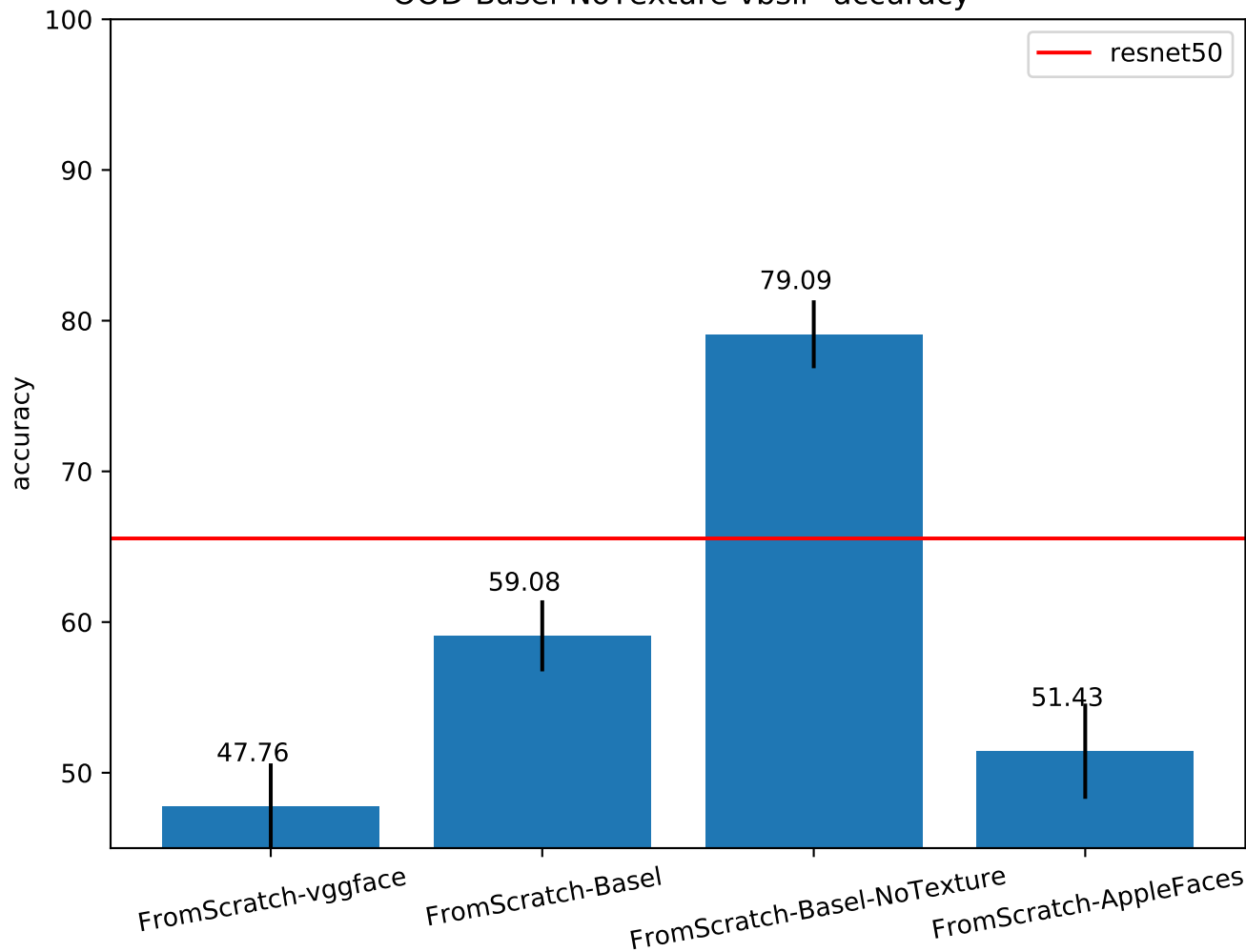
OOD-Basel-NoTexture vbsli* accuracy
