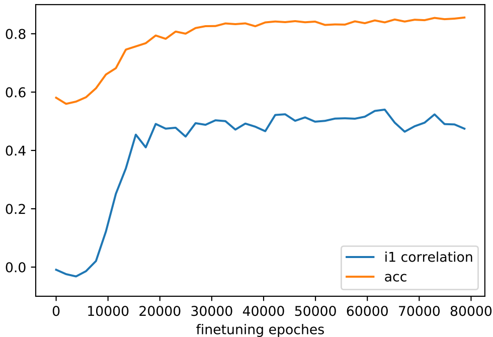
finetuning for AppleFaces
