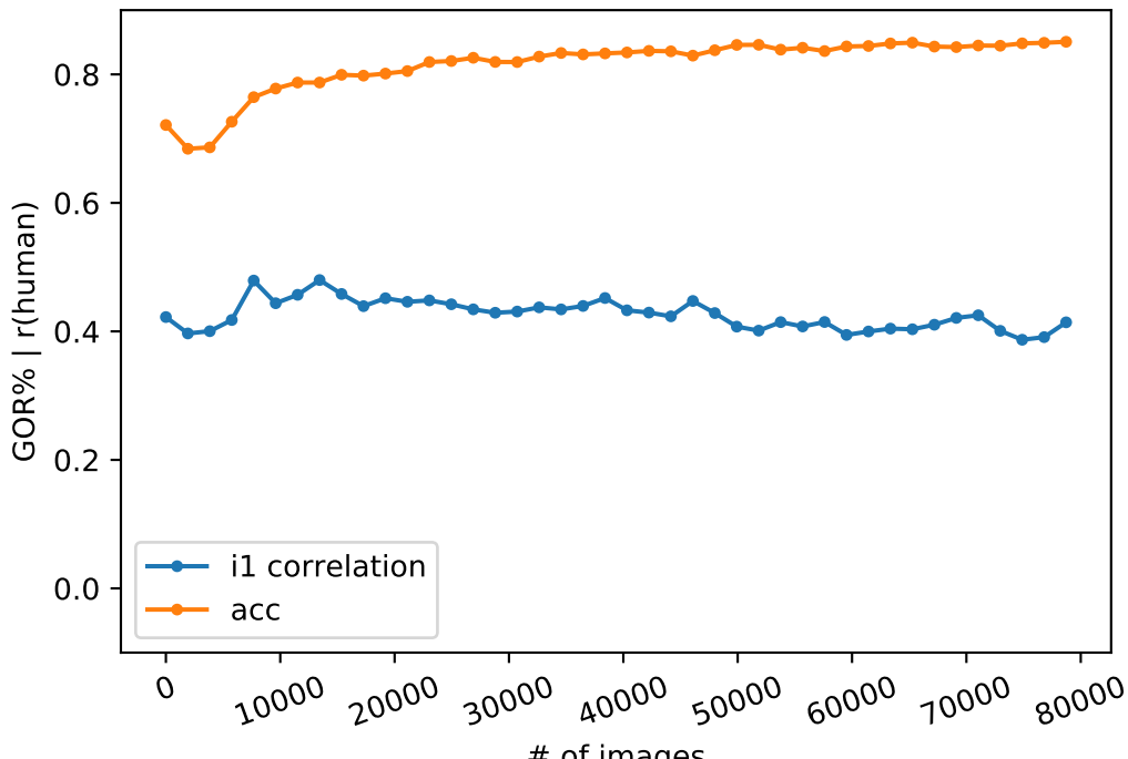
Camel-Elephant fine-tuning, 1 epoch
