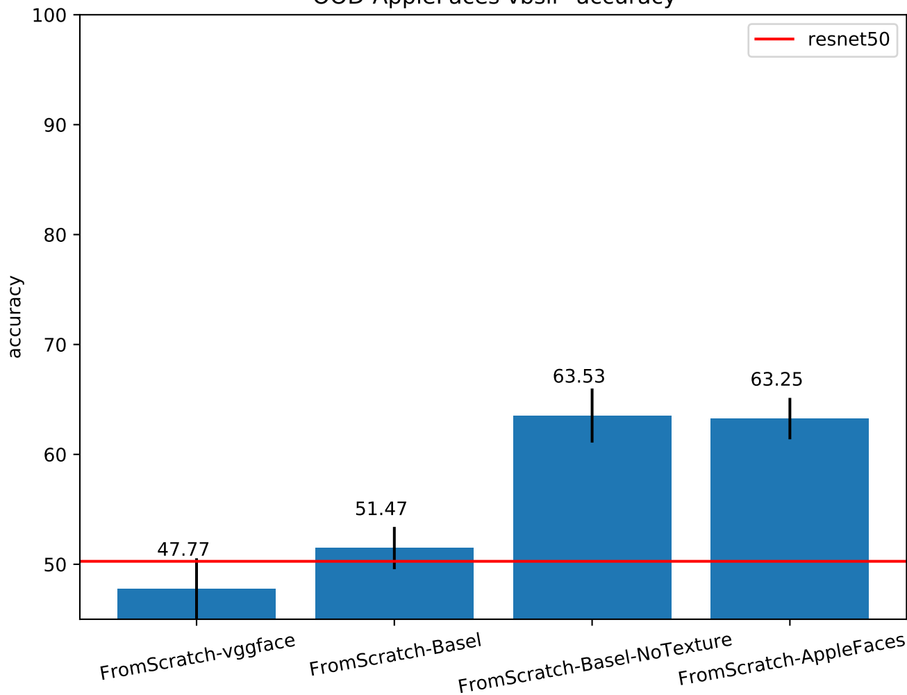
OOD-AppleFaces vbsli* accuracy
