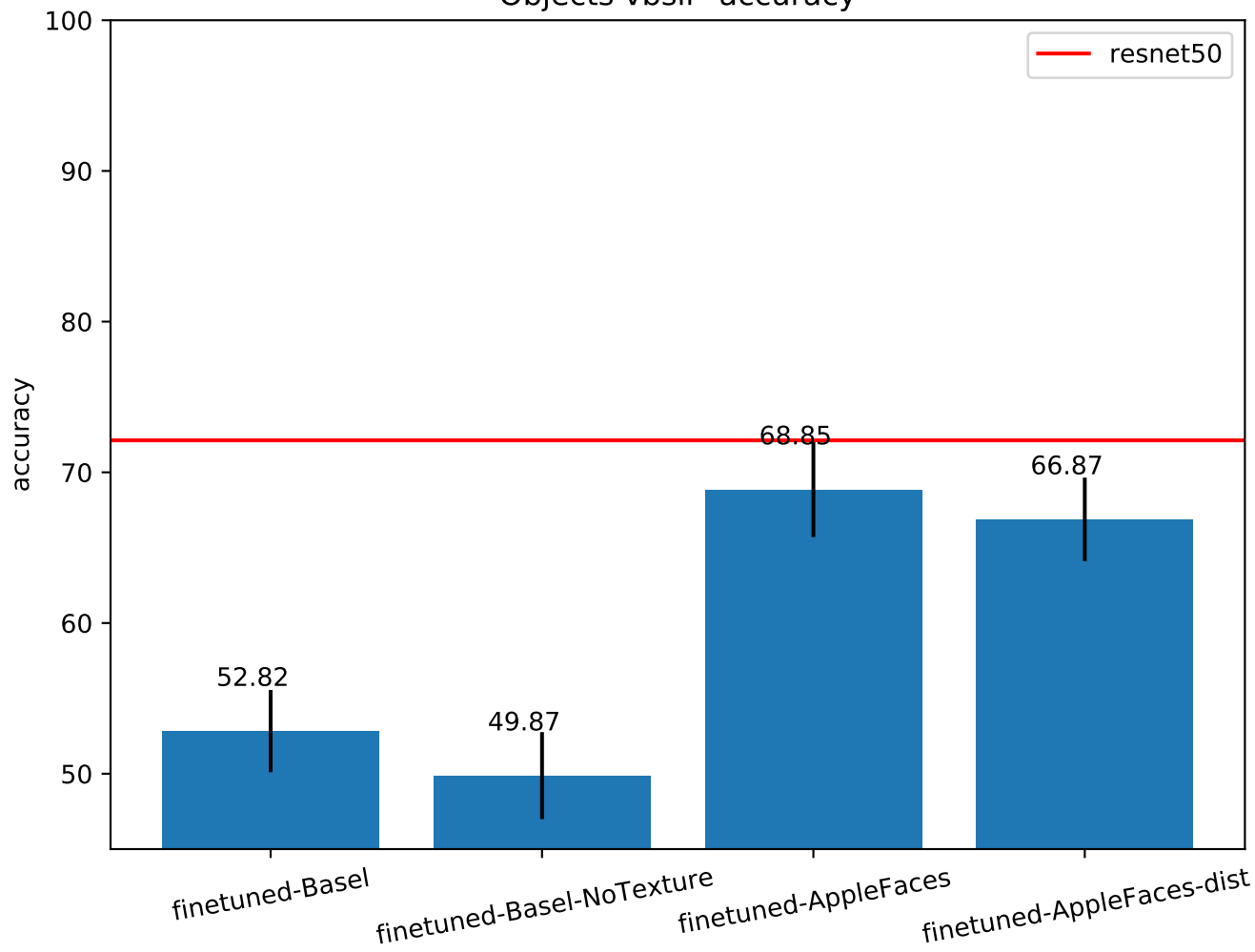
Objects vbsli* accuracy
