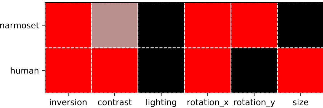
Regression analysis of latent variables vs. i1
