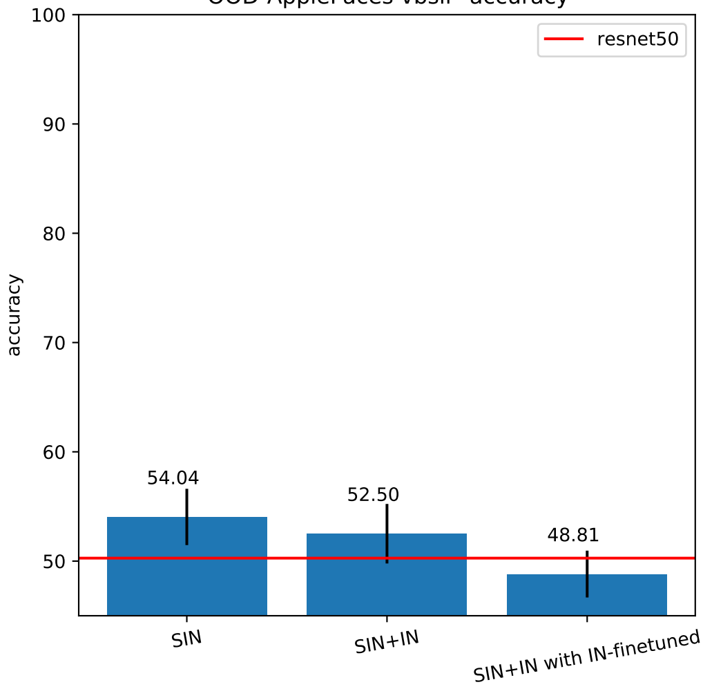
OOD-AppleFaces vbsli* accuracy
