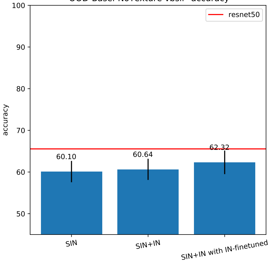
OOD-Basel-NoTexture vbsli* accuracy
