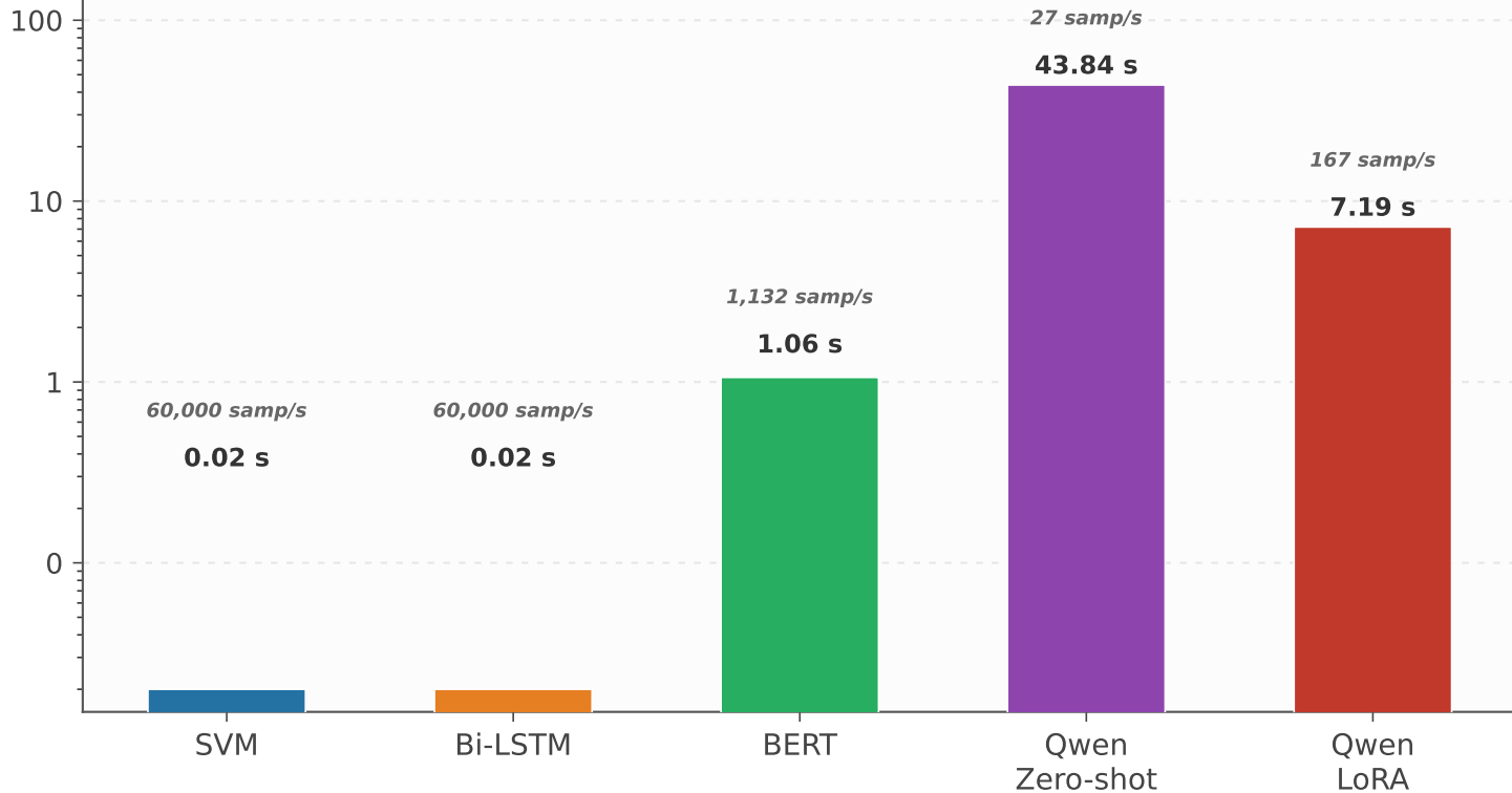
Inference Time (s, log scale)
